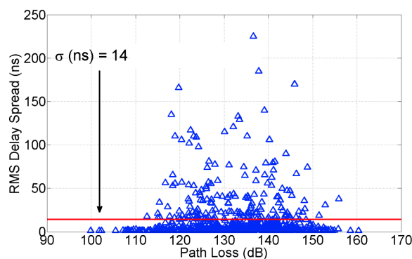
FIGURE 18. RMS delay spread as a function of path loss over all viable pointing angles at 38 GHz in Austin, Texas. The blue triangles represent the measured RMS delay spread, and the red line denotes a linear fit for the average RMS delay spread.
