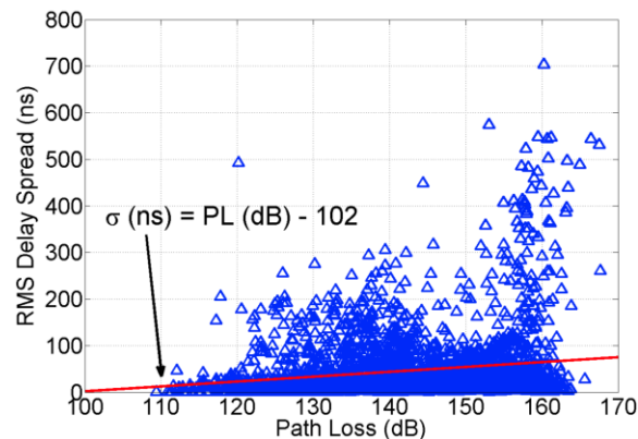
FIGURE 17. RMS delay spread as a function of path loss over all viable pointing angles at 28 GHz in New York City. The blue triangles represent the measured RMS delay spread and the red line denotes a linear fit for the average RMS delay spread.
