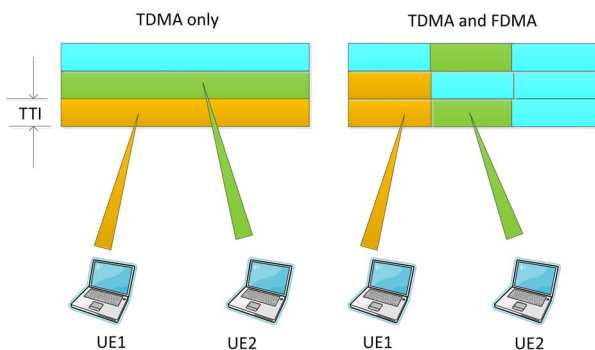
Fig. 13. Multiple access: Enabling FDMA (within a TDD time slot), where multiple UEs can be scheduled at a time, can offer numerous benefits in mmW systems, including improved power in the uplink, more efficient transmission of small packets, and reduced UE power consumption. A key design issue is how to support FDMA in TDD with mmW front-ends that perform beamsteering in analog.
