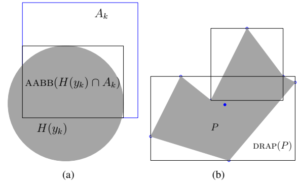
Fig. 3. (a) Computing O_{\text{rect}}(A_k, y_k) to find the rectangle approximated I-state, given an observation y_k . (b) Algorithm 1 returns a double rectangle \text{DRAP}(P) around the given input polygon P .
