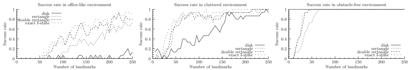
Fig. 4. Success rate versus number of landmarks for the environments in Figures 6-8.
