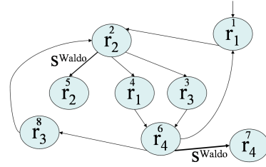
Fig. 2: The synthesized automaton of Example 2
