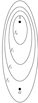
Figure 1: f -cost diagram for A* and IDA*
