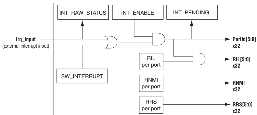
Figure 31-3. Interrupt Request Block
