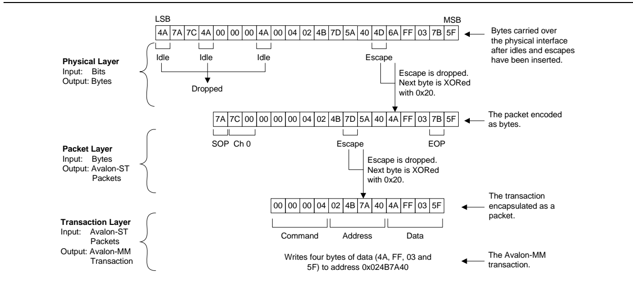
Figure 18-3. Bits to Avalon-MM Transaction
