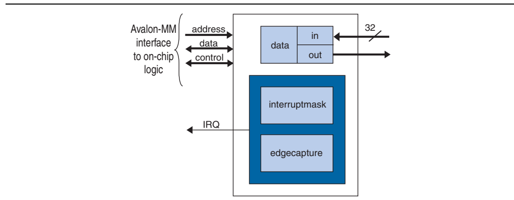
Figure 10–2. PIO Core with Input Ports, Output Ports, and IRQ Support
