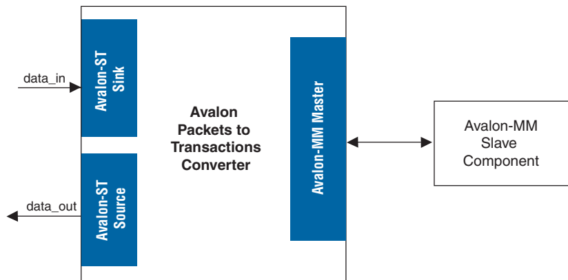
Figure 21–1. Avalon Packets to Transactions Converter Core
