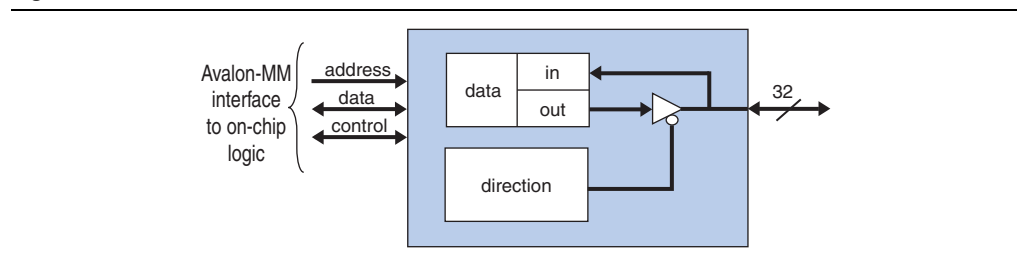
Figure 10–3. PIO Core with Bidirectional Ports
