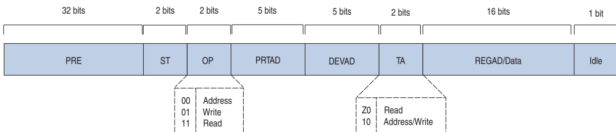
Figure 14-2. MDIO Frame Format (Clause 45)
