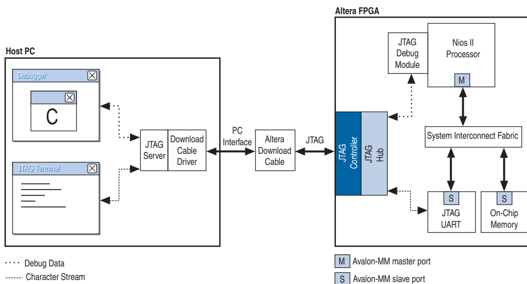
Figure 6-2. Example System Using the JTAG UART Core
