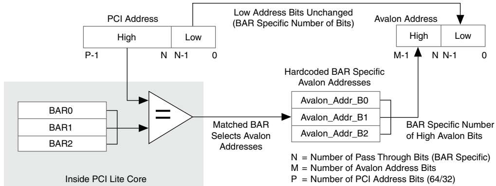
Figure 12-2. PCI-to-Avalon Address Translation
