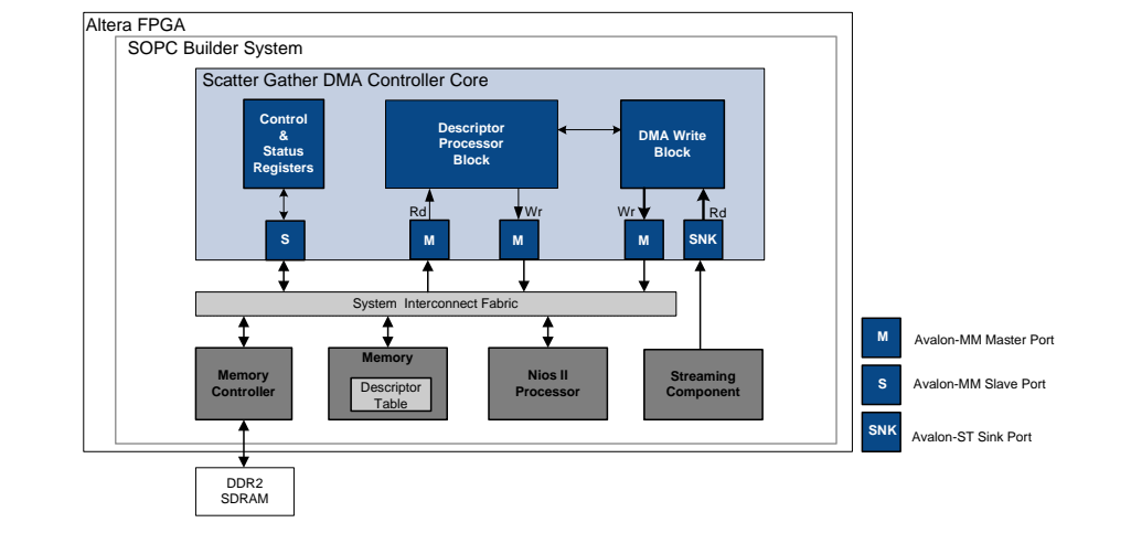
Figure 25–1. SG-DMA Controller Core with Streaming Peripheral and External Memory
