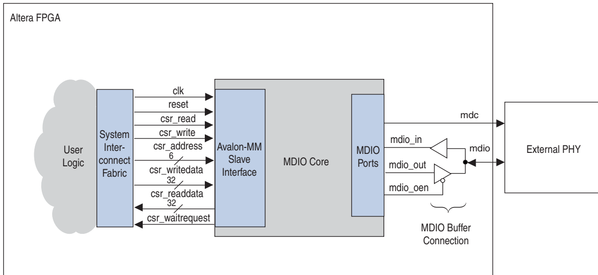
Figure 14-1. MDIO Core Block Diagram
