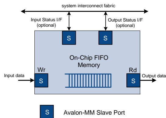
Figure 16-1. FIFO with Avalon-MM Input and Output Interfaces
