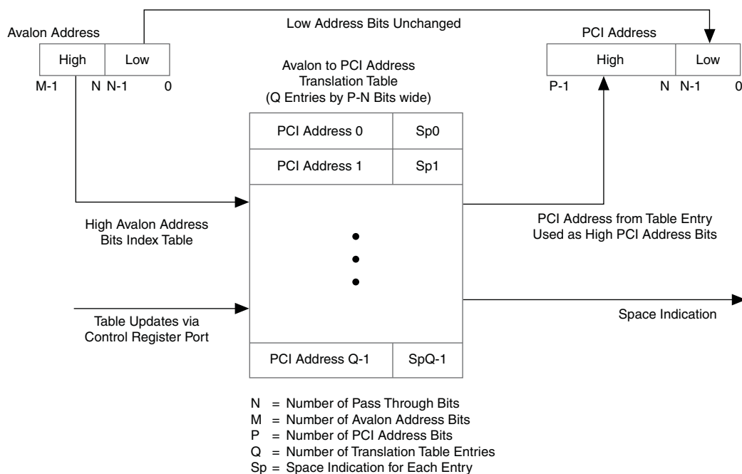
Figure 12-3. Avalon-to-PCI Address Translation
