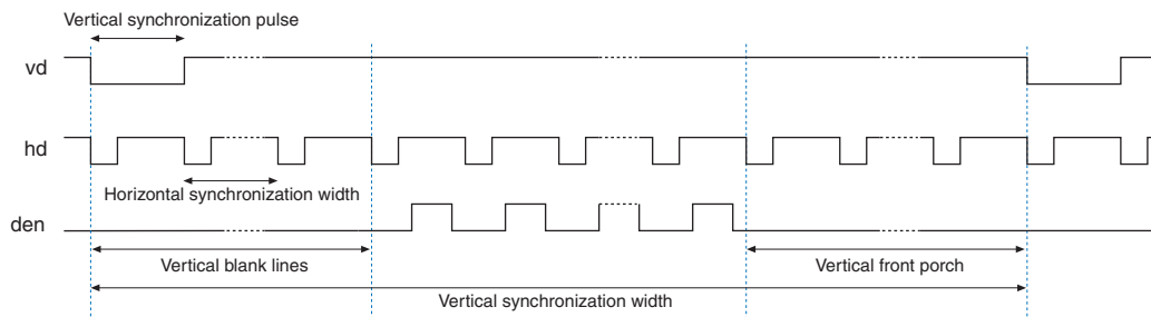
Figure 27-5. Vertical Synchronization Timing—8 Bits DataWidth and 3 Beats Per Pixel / 24 Bits DataWidth and 1 Beat Per Pixel
