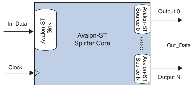
Figure 24–1. Avalon-ST Splitter Core
