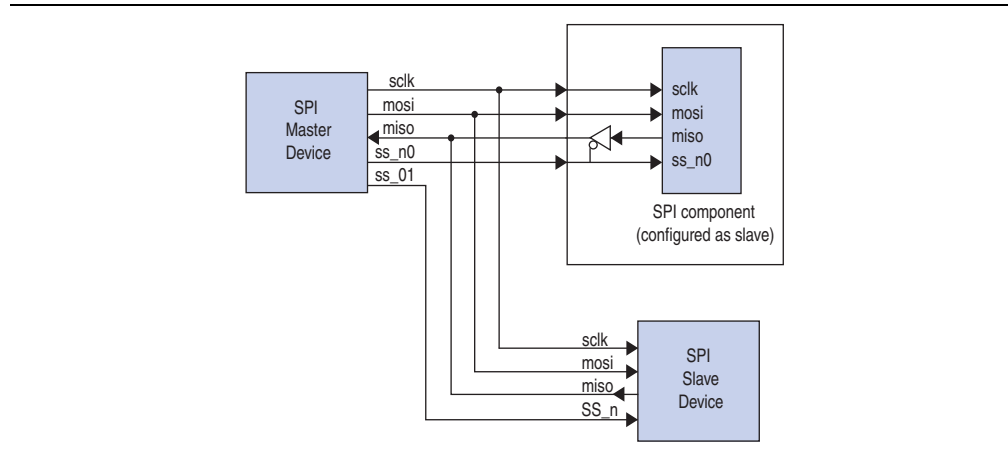
Figure 8-3. SPI Core in a Multi-Slave Environment
