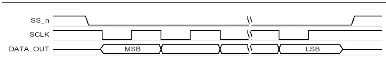
Figure 8-8. Clock Polarity = 1, Clock Phase = 1
