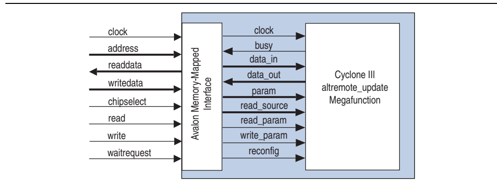
Figure 13–1. Cyclone III Remote Update Controller Core Block Diagram
