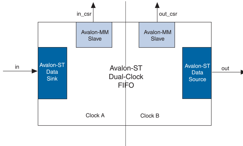
Figure 15-2. Avalon-ST Dual Clock FIFO Core
