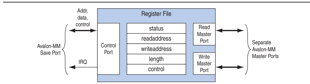
Figure 26-1. DMA Controller Block Diagram
