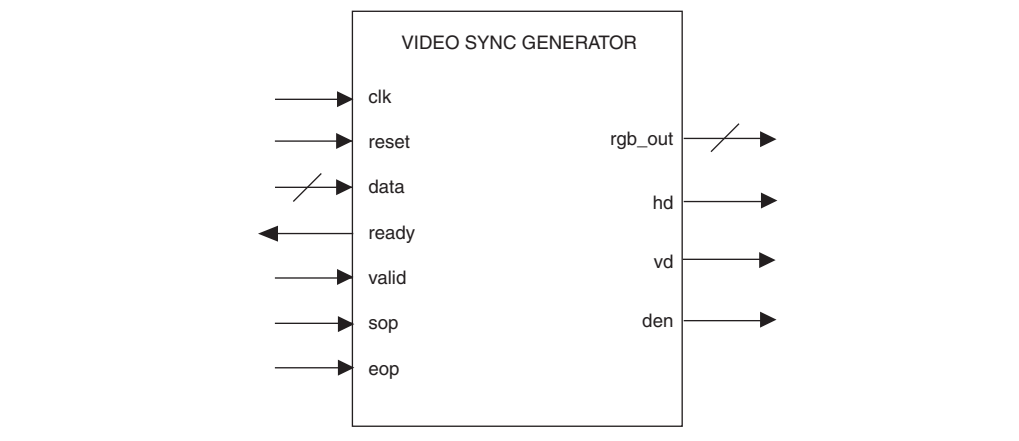
Figure 27-2. Video Sync Generator Block Diagram
