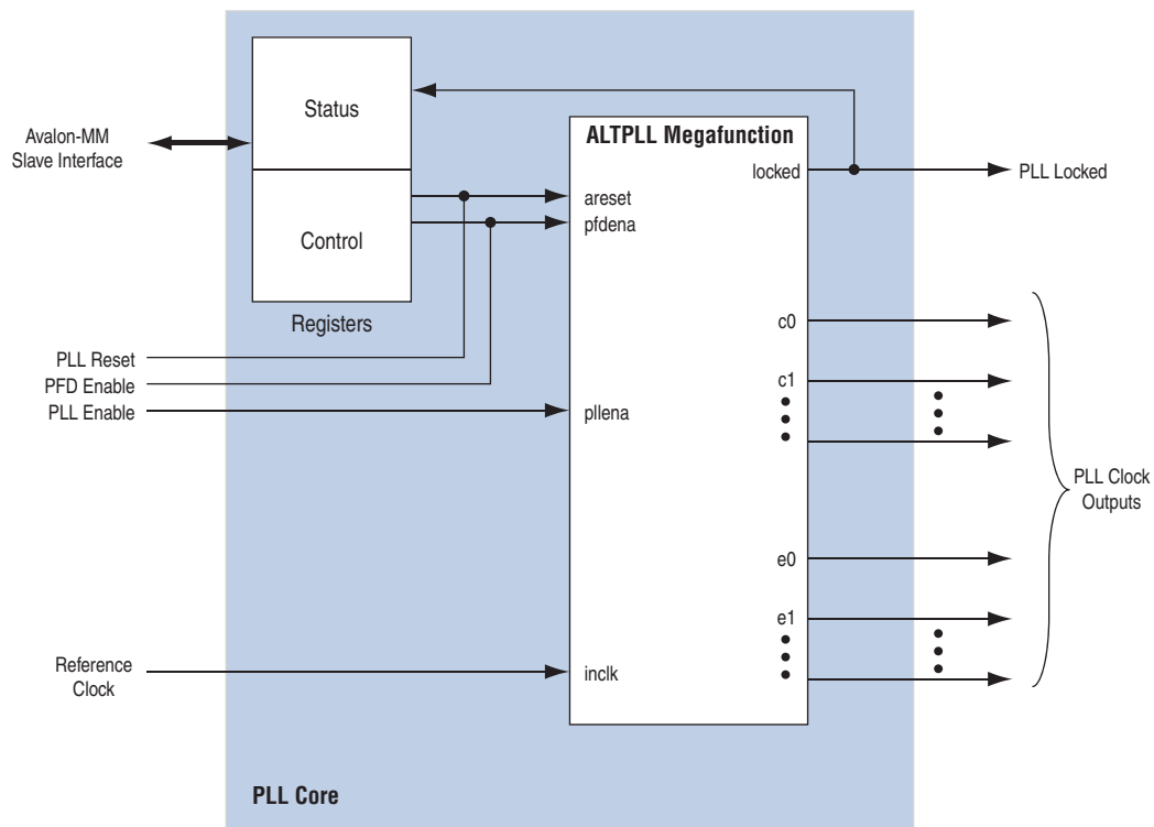
Figure 37-1. PLL Core Block Diagram
