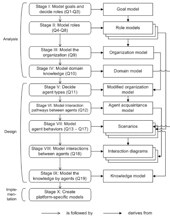
Fig. 1. The software engineering process for designing societal information systems.
