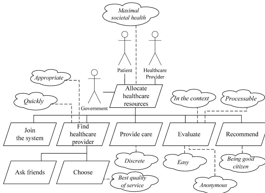
Fig. 8. The goal model of the societal healthcare information system.
