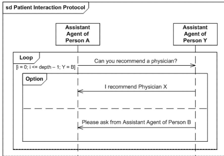
Fig. 12. The interaction protocol between patients' Assistant Agents.
