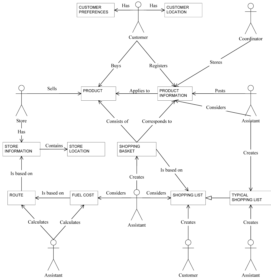
Fig. 5. The elaborated domain model of the societal information system of grocery shopping.
