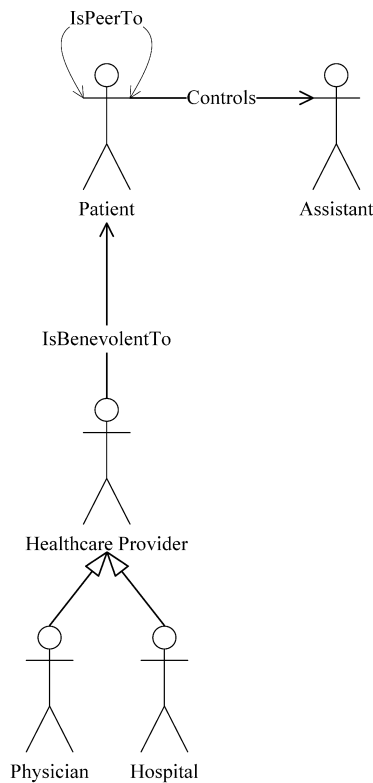
Fig. 9. The organization model of the societal healthcare information system.
