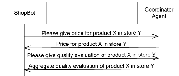
Fig. 7. A message sequence between ShopBot and Coordinator Agent.
