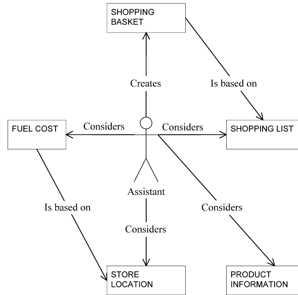
Fig. 4. Partial domain model of the societal information system of grocery shopping.
