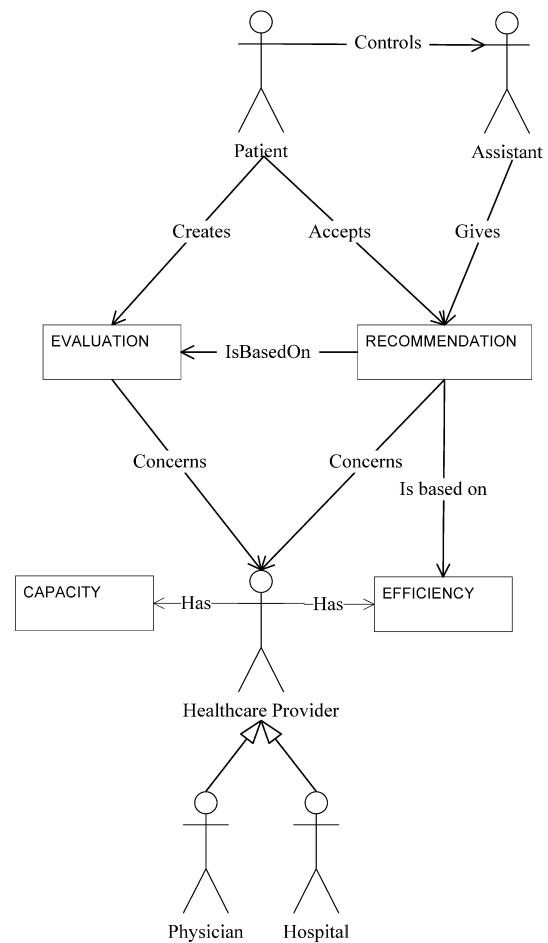
Fig. 10. The domain model of the societal information system of healthcare.
