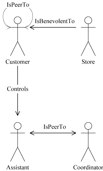
Fig. 3. The organization model of societal information system of grocery shopping.
