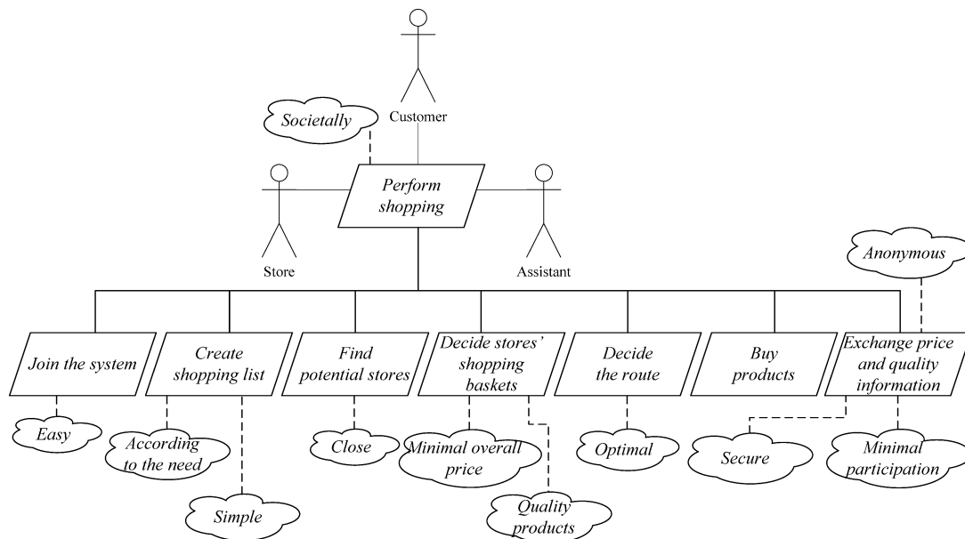
Fig. 2. The overall goal model for a societal information system of grocery shopping.
