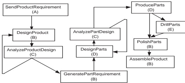
Figure 2: A ProduceProduct Workflow Example
