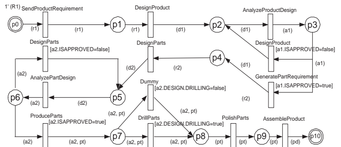
Figure 4: A ProduceProduct Petri Net
