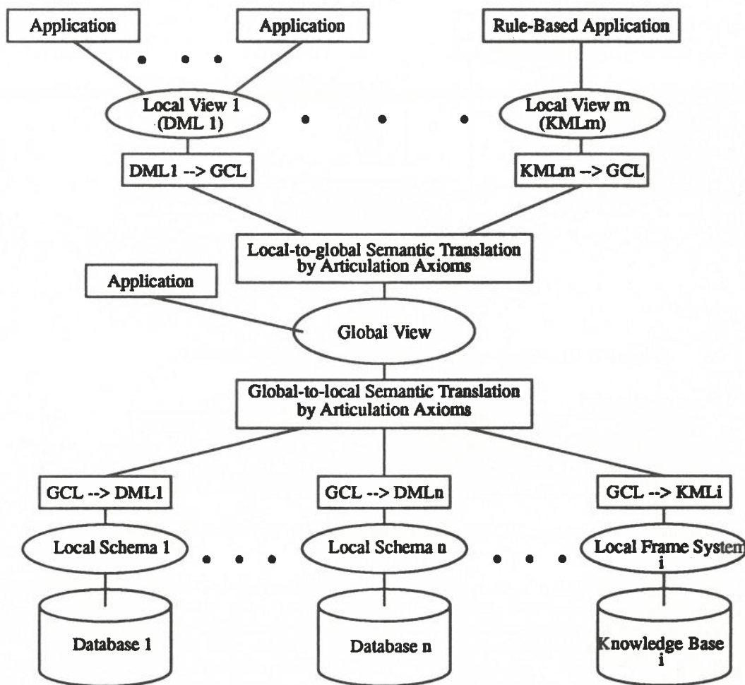
Figure 1: Global and local views in semantic transaction processing
