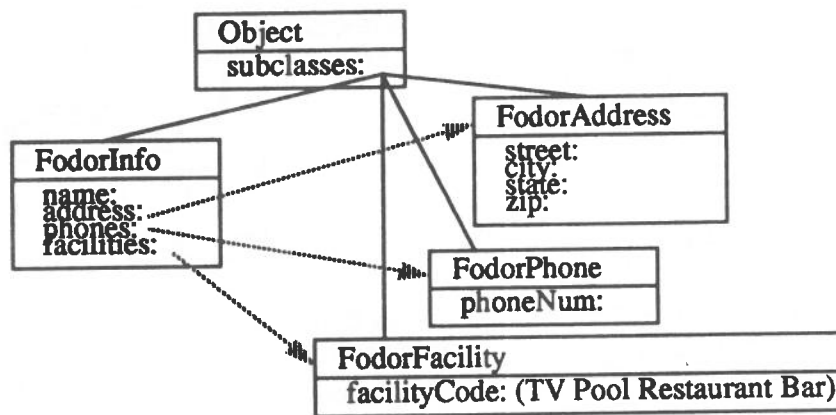
Figure 2: The object-oriented schema for the Fodor database
