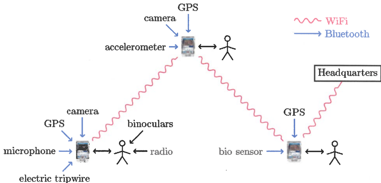
Fig. 5. Schematic view of handheld advisors' (ACTAR's) deployment
