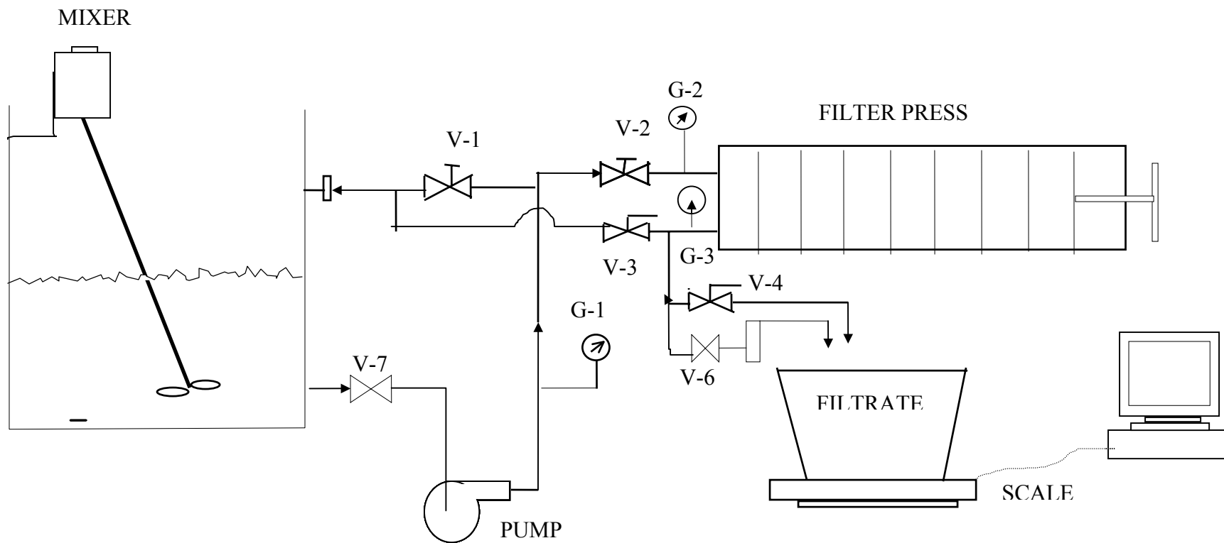
FIGURE 1 FILTRATION EQUIPMENT FLOWSHEET
