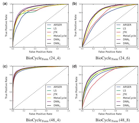
Fig. 6. ROC Curves of different methods on the \text{BioCycle}_{\text{Form}} dataset
