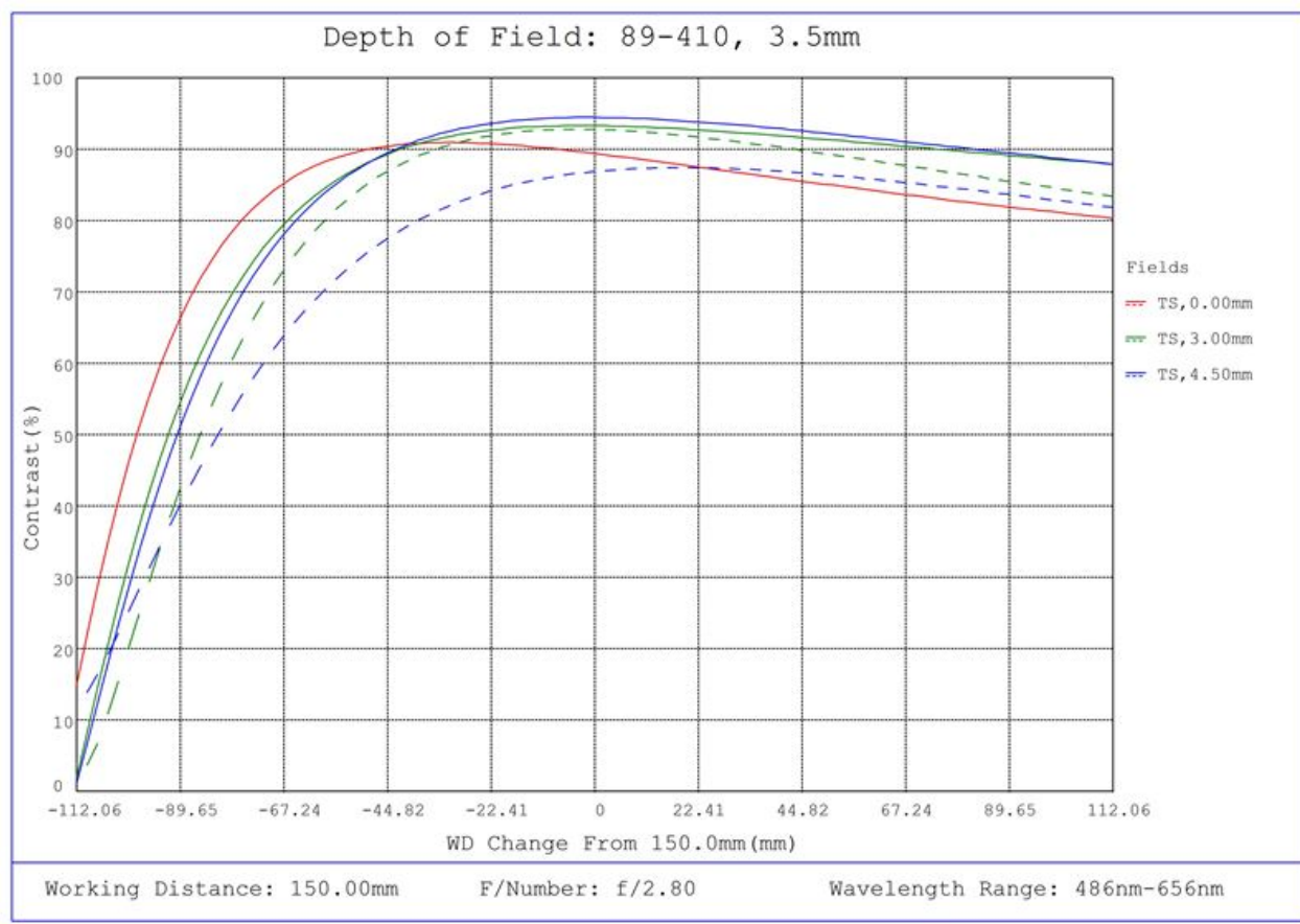
#89-410, 3.5mm C Series Fixed Focal Length Lens, Depth of Field Plot, 150mm Working Distance, f2.8
