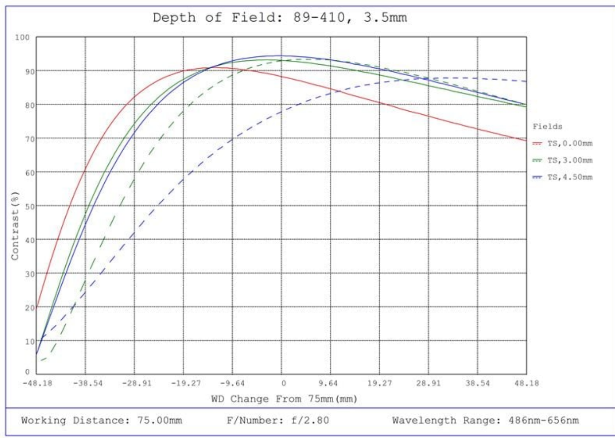
#89-410, 3.5mm C Series Fixed Focal Length Lens, Depth of Field Plot, 75mm Working Distance, f2.8
