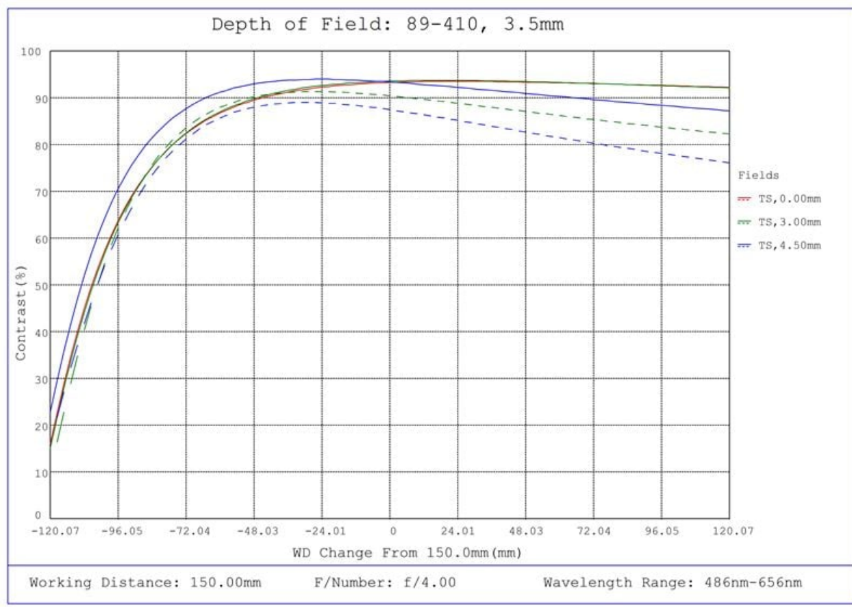
#89-410, 3.5mm C Series Fixed Focal Length Lens, Depth of Field Plot, 150mm Working Distance, f4
