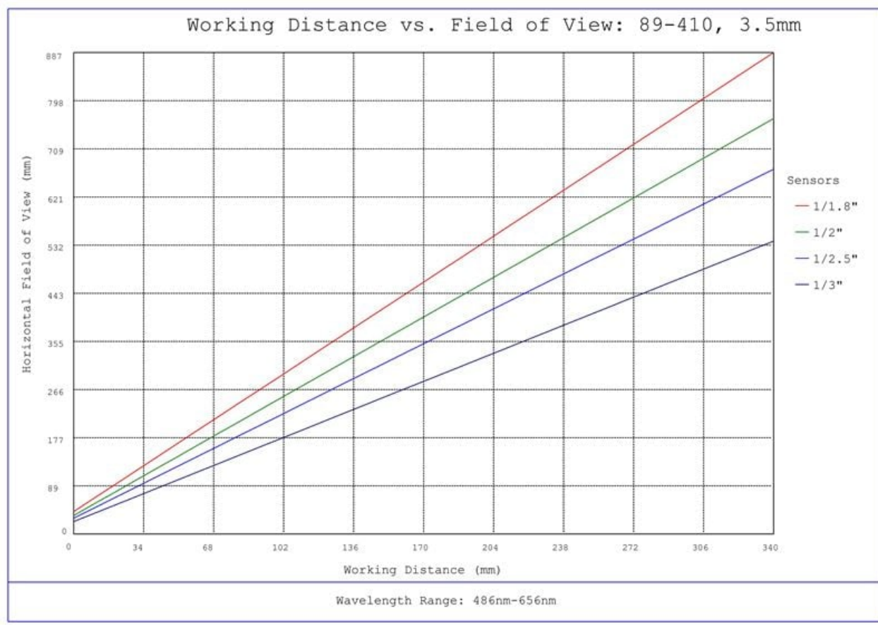
#89-410, 3.5mm C Series Fixed Focal Length Lens, Working Distance versus Field of View Plot
