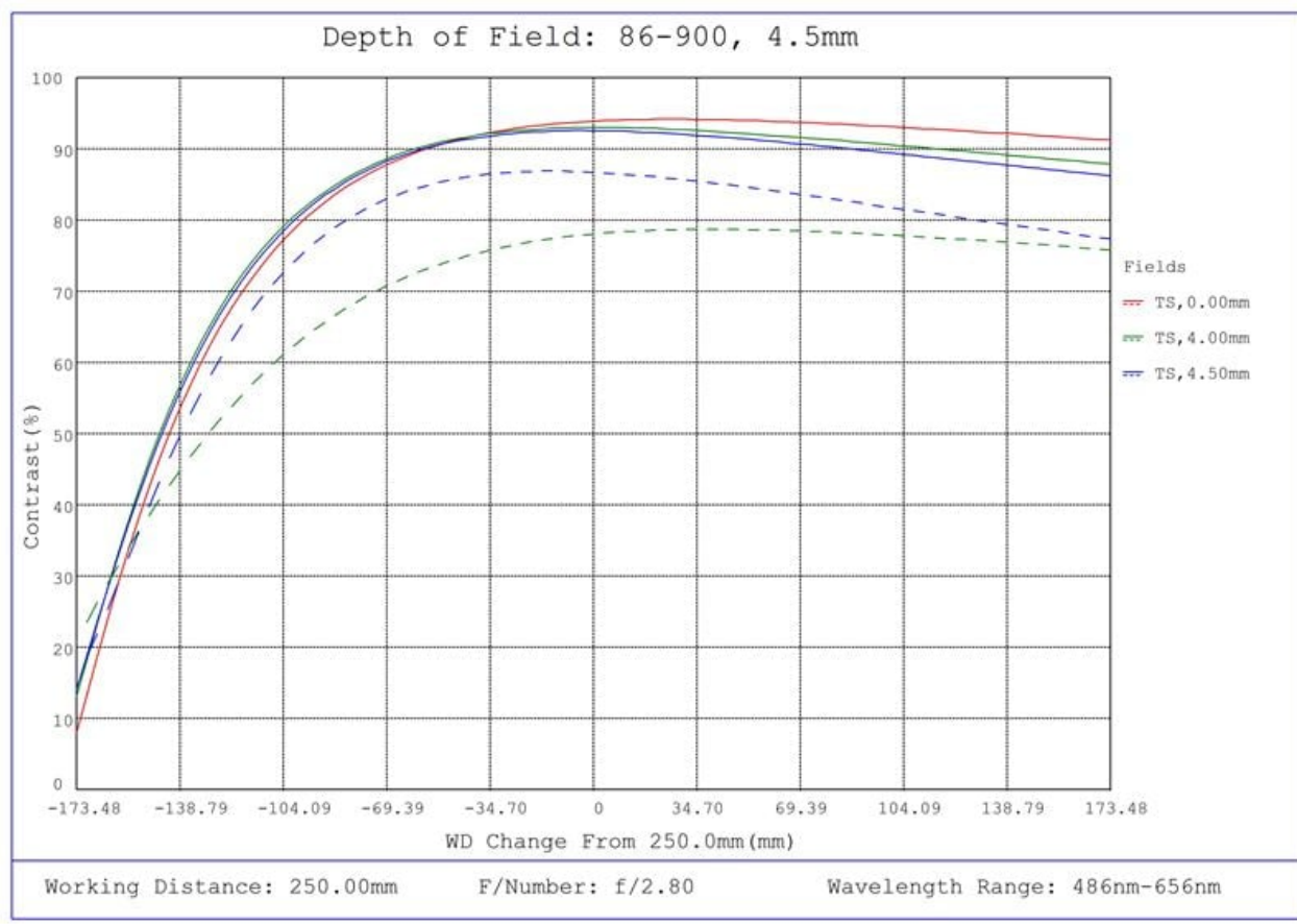
#86-900, 4.5mm C Series Fixed Focal Length Lens, Depth of Field Plot, 250mm Working Distance, f2.8
