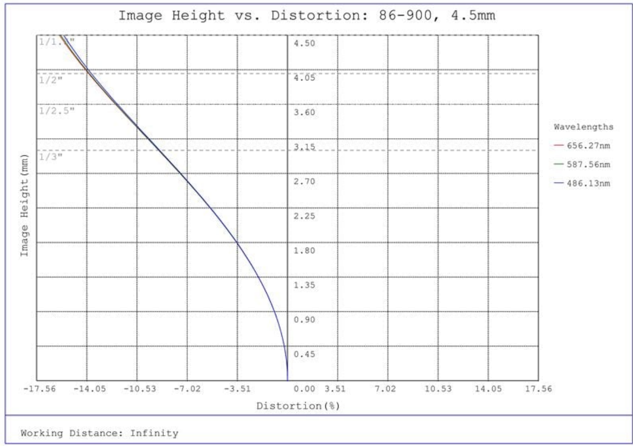
#86-900, 4.5mm C Series Fixed Focal Length Lens, Distortion Plot
