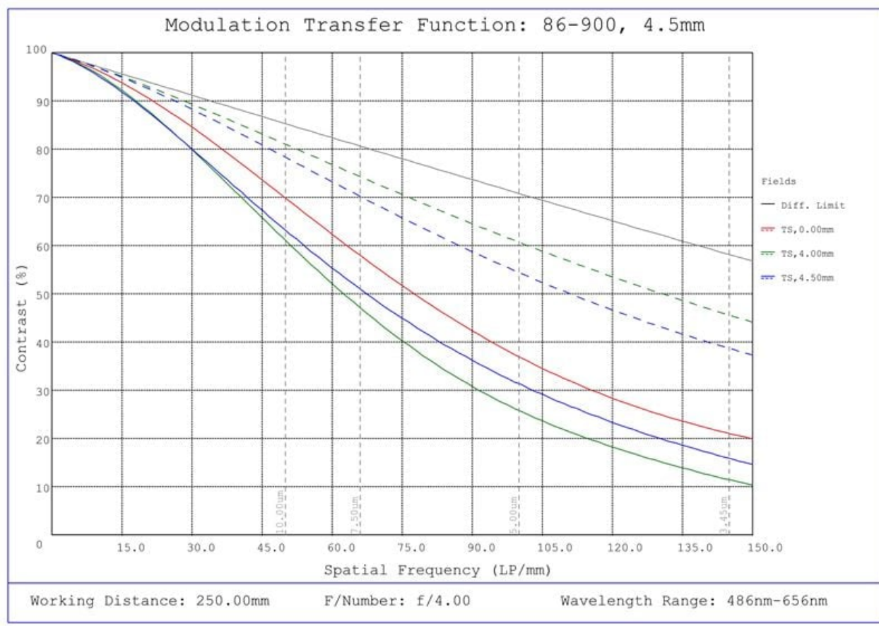
#86-900, 4.5mm C Series Fixed Focal Length Lens, Modulated Transfer Function (MTF) Plot, 250mm Working Distance, f4
