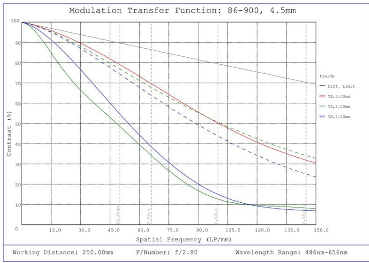
#86-900, 4.5mm C Series Fixed Focal Length Lens, Modulated Transfer Function (MTF) Plot, 250mm Working Distance, f2.8
