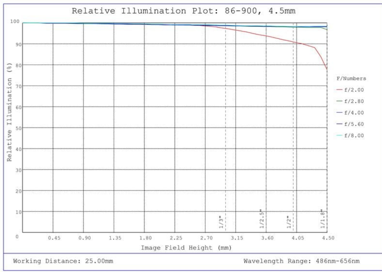
#86-900, 4.5mm C Series Fixed Focal Length Lens, Relative Illumination Plot
