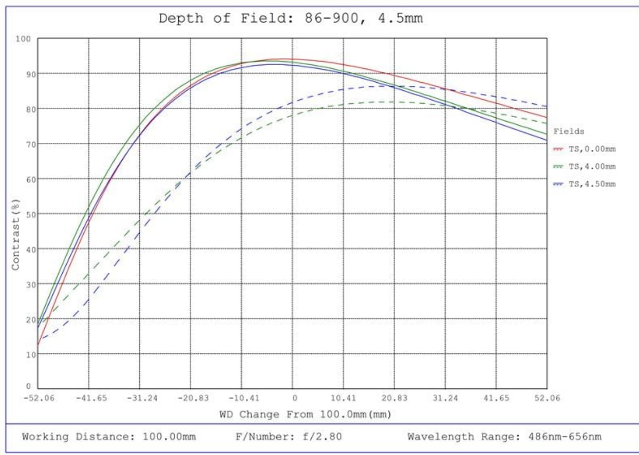
#86-900, 4.5mm C Series Fixed Focal Length Lens, Depth of Field Plot, 100mm Working Distance, f2.8
