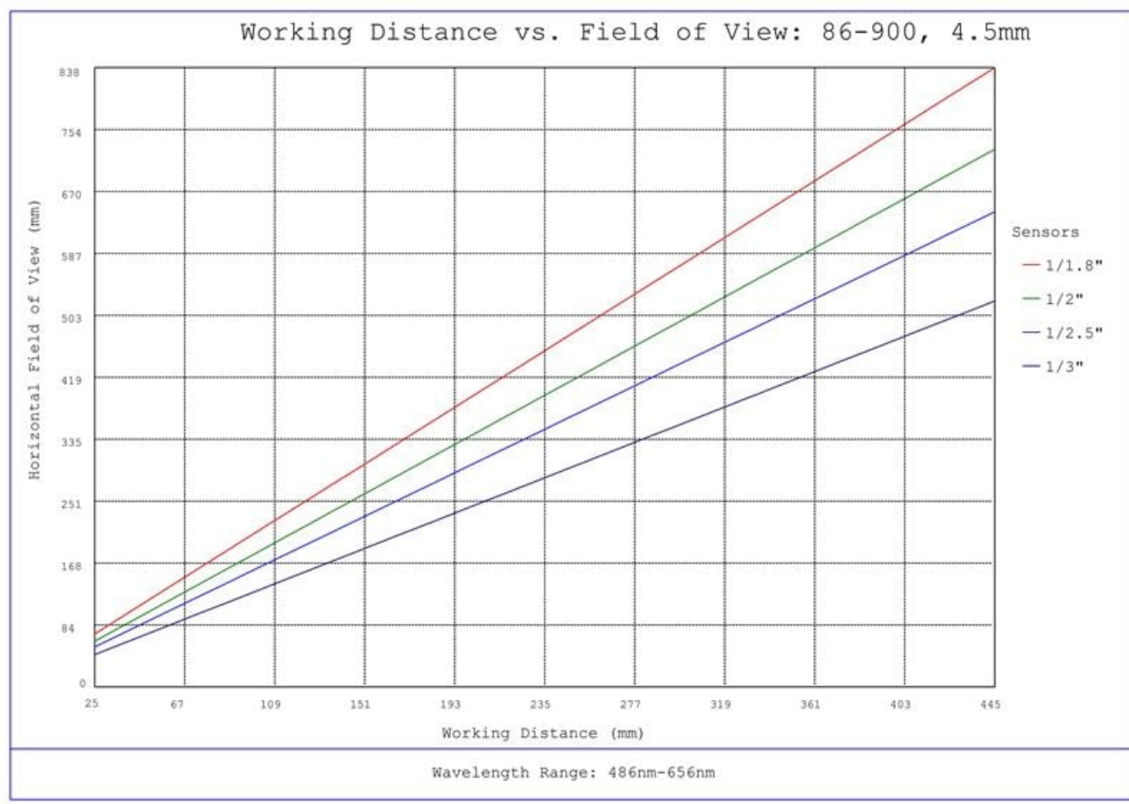
#86-900, 4.5mm C Series Fixed Focal Length Lens, Working Distance versus Field of View Plot
