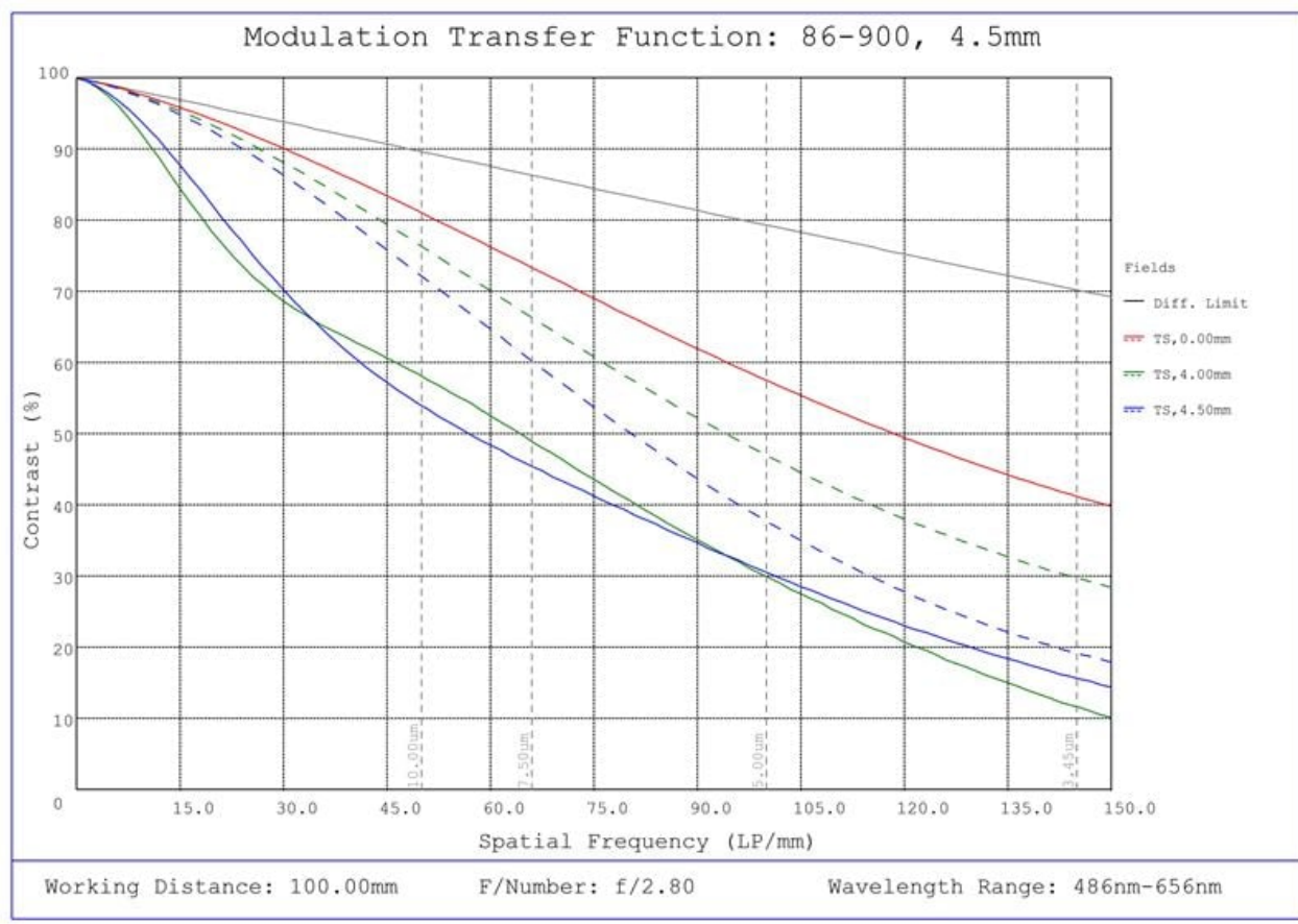
#86-900, 4.5mm C Series Fixed Focal Length Lens, Modulated Transfer Function (MTF) Plot, 100mm Working Distance, f2.8
