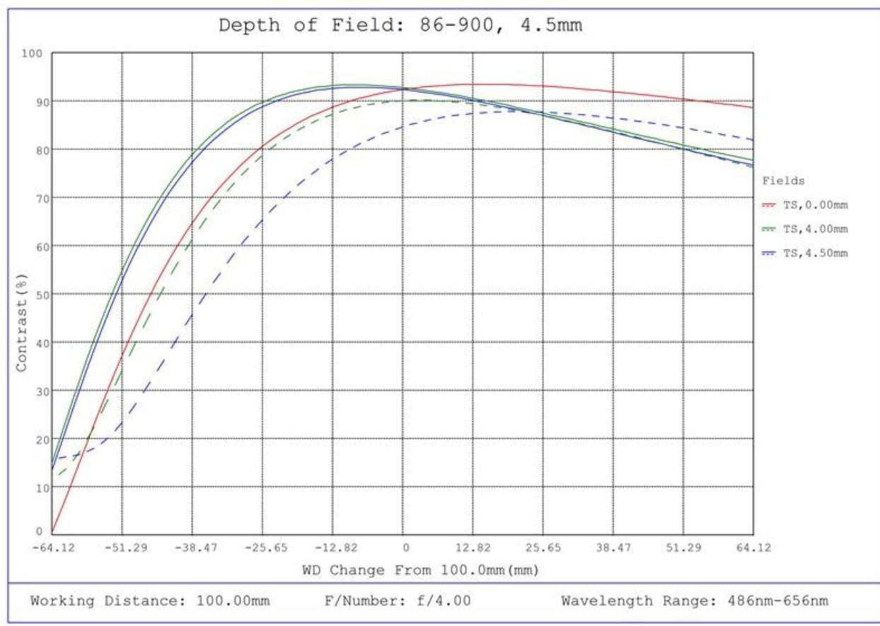
#86-900, 4.5mm C Series Fixed Focal Length Lens, Depth of Field Plot, 100mm Working Distance, f4
