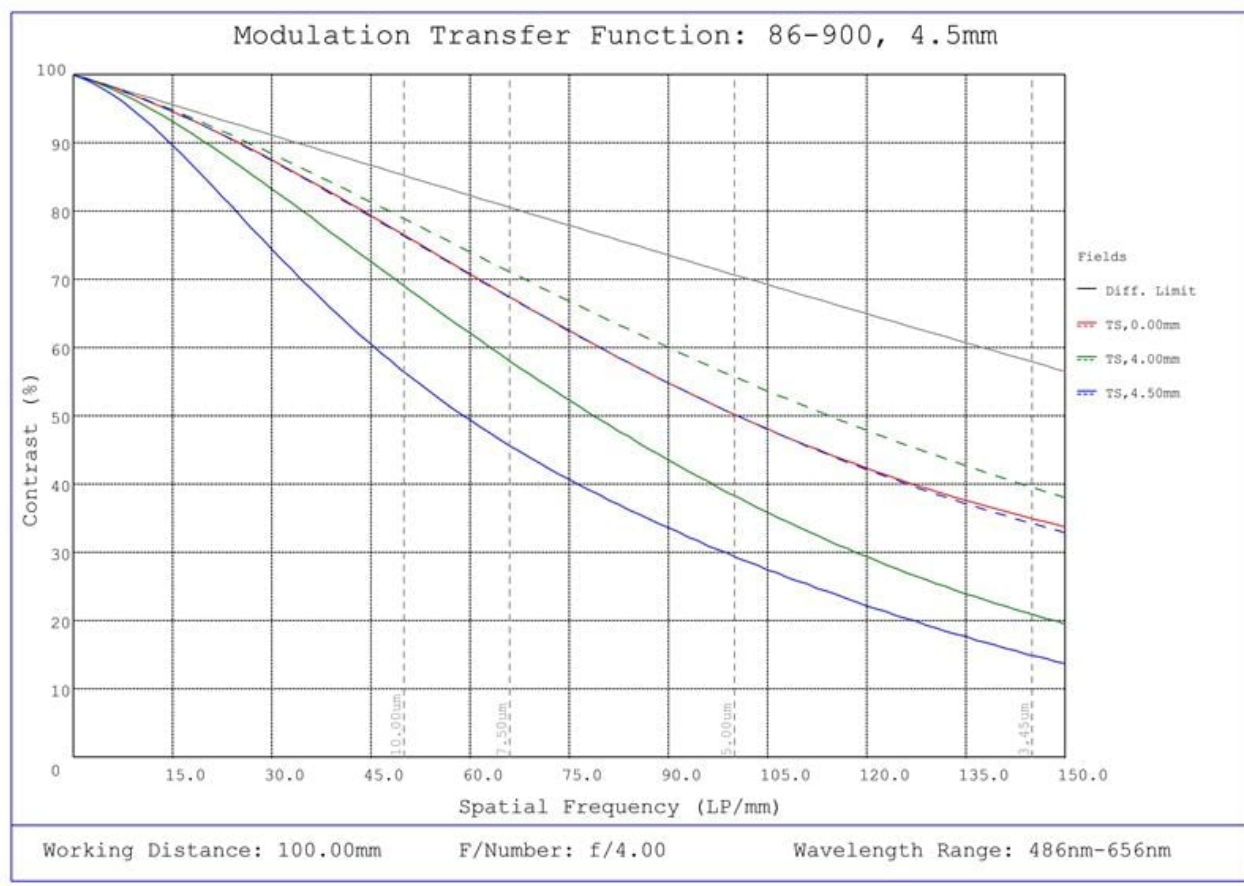
#86-900, 4.5mm C Series Fixed Focal Length Lens, Modulated Transfer Function (MTF) Plot, 100mm Working Distance, f4
