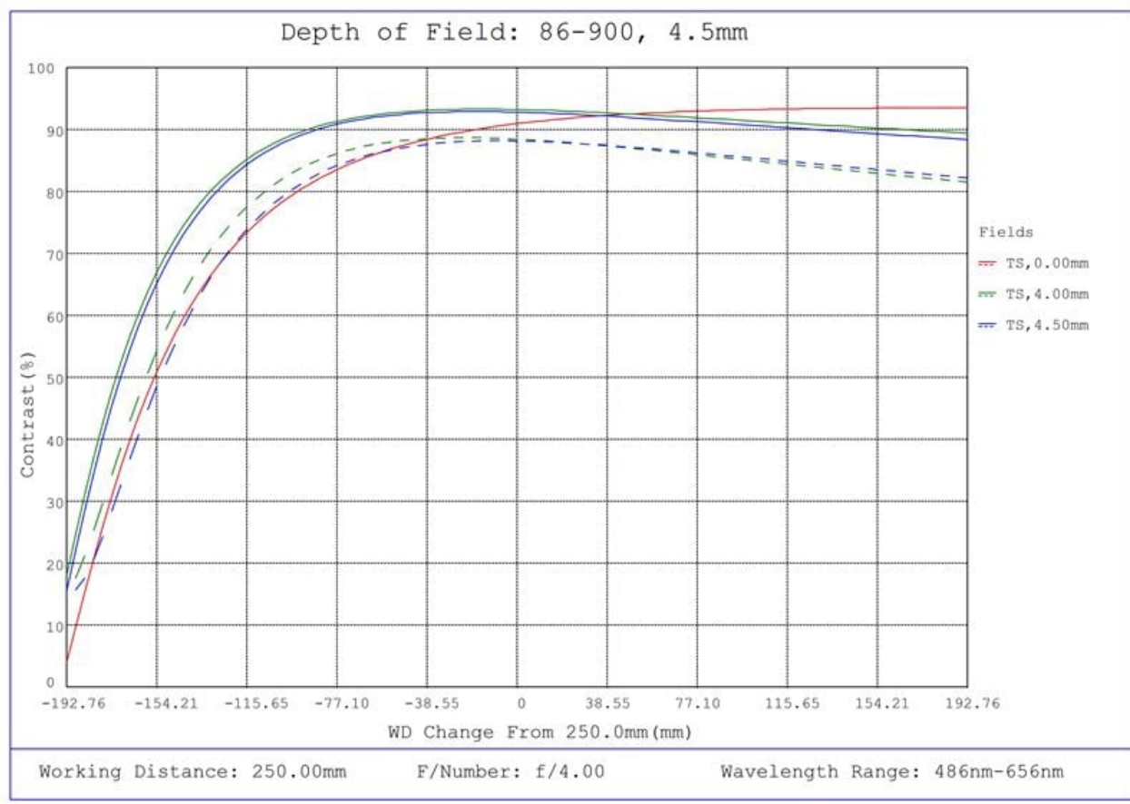
#86-900, 4.5mm C Series Fixed Focal Length Lens, Depth of Field Plot, 250mm Working Distance, f4
