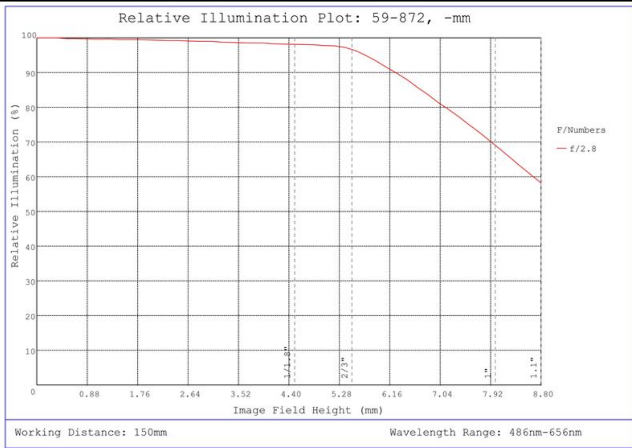
#59-872, 35mm C Series Fixed Focal Length Lens, Relative Illumination Plot
