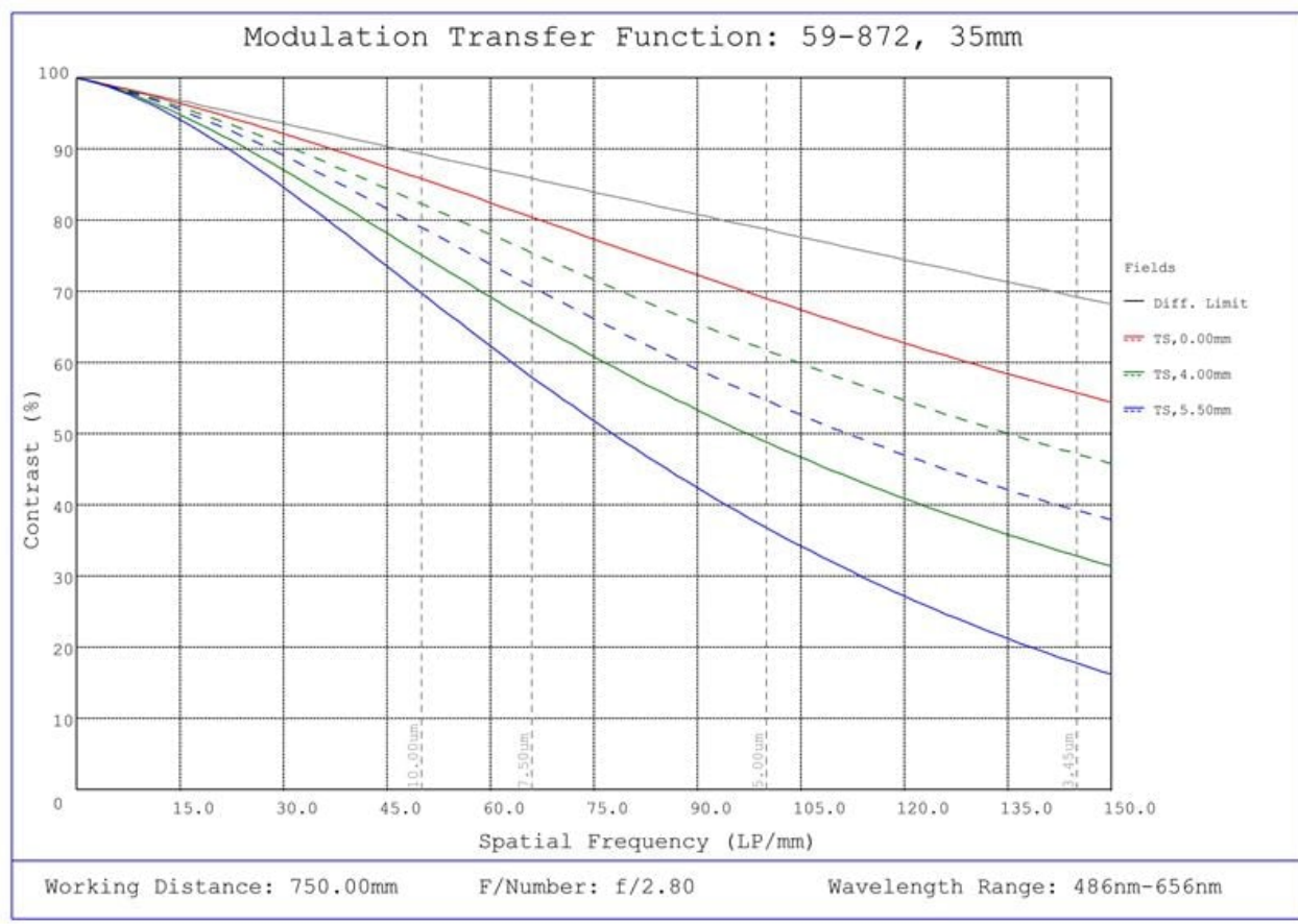
#59-872, 35mm C Series Fixed Focal Length Lens, Modulated Transfer Function (MTF) Plot, 750mm Working Distance, f2.8
