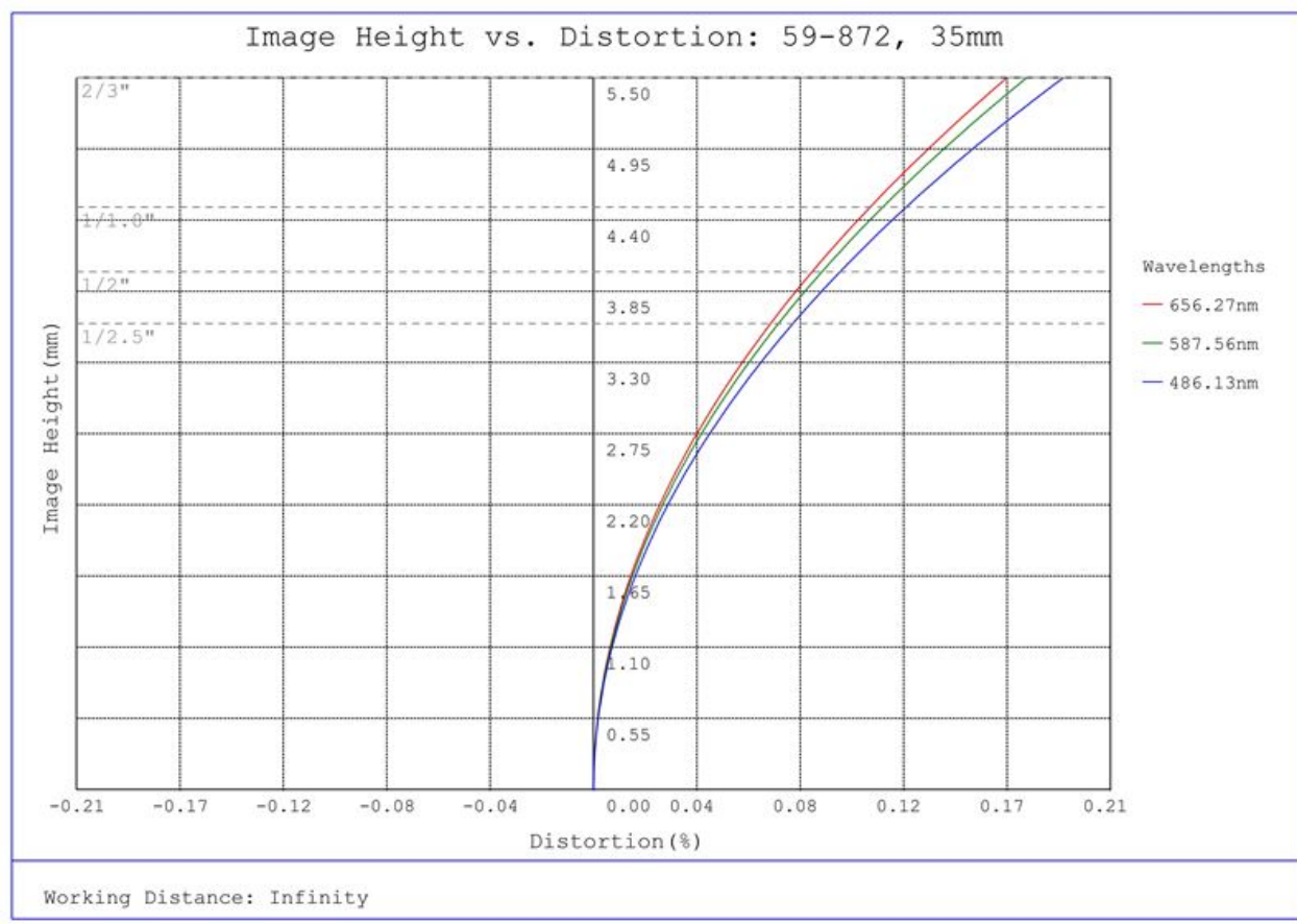
#59-872, 35mm C Series Fixed Focal Length Lens, Distortion Plot
