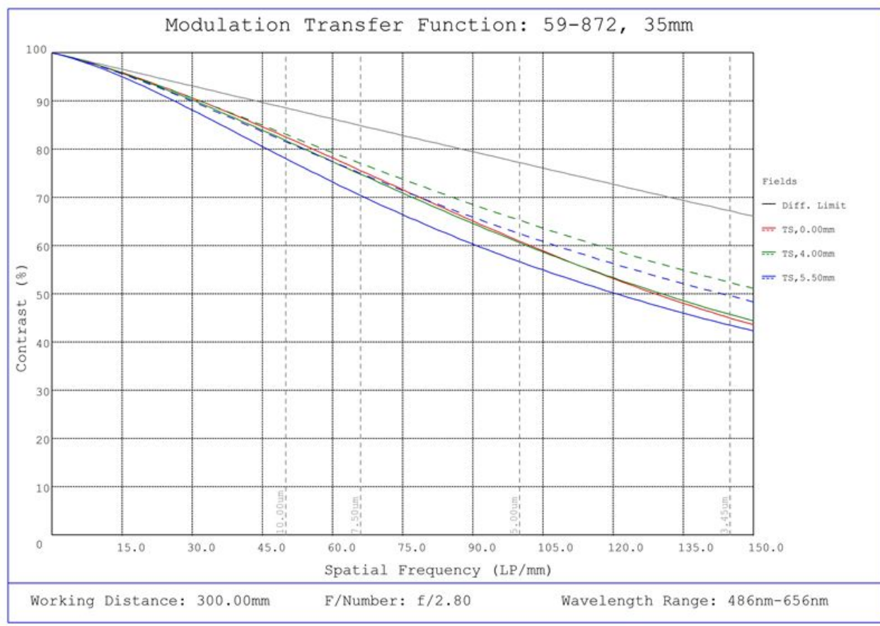
#59-872, 35mm C Series Fixed Focal Length Lens, Modulated Transfer Function (MTF) Plot, 300mm Working Distance, f2.8
