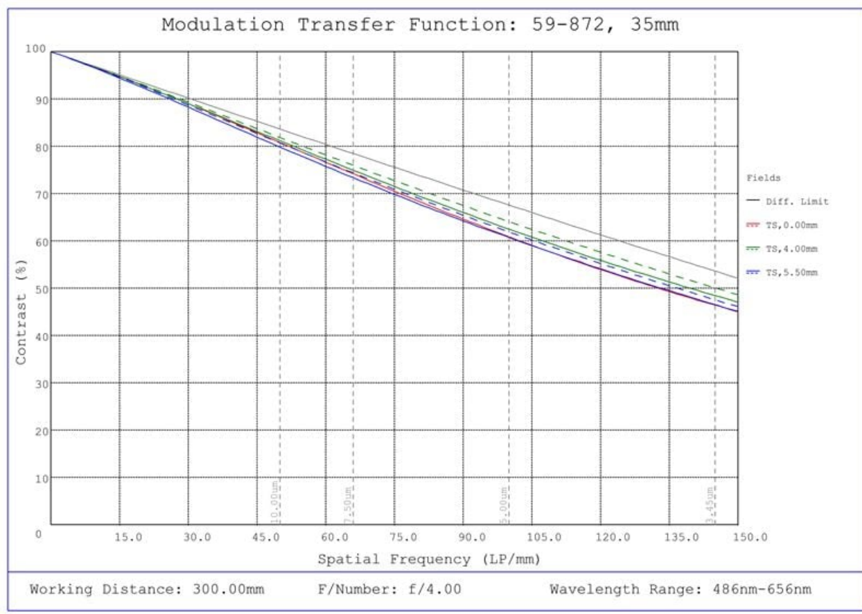
#59-872, 35mm C Series Fixed Focal Length Lens, Modulated Transfer Function (MTF) Plot, 300mm Working Distance, f4
