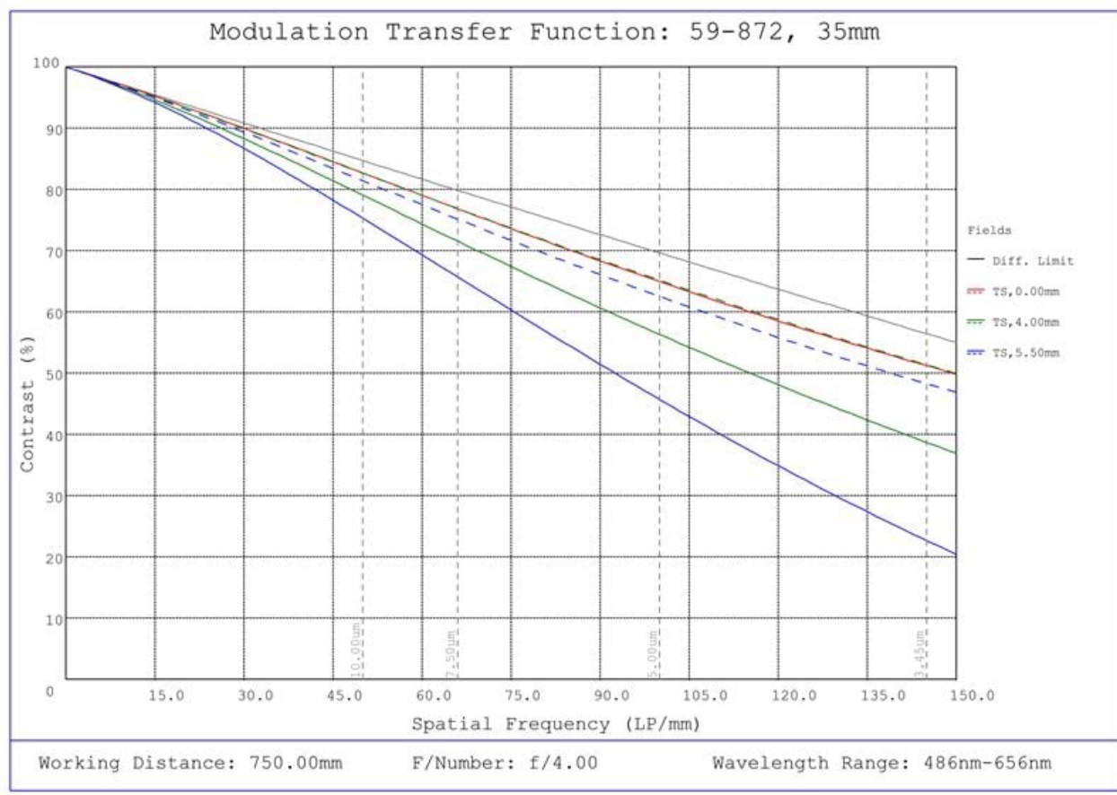
#59-872, 35mm C Series Fixed Focal Length Lens, Modulated Transfer Function (MTF) Plot, 750mm Working Distance, f4
