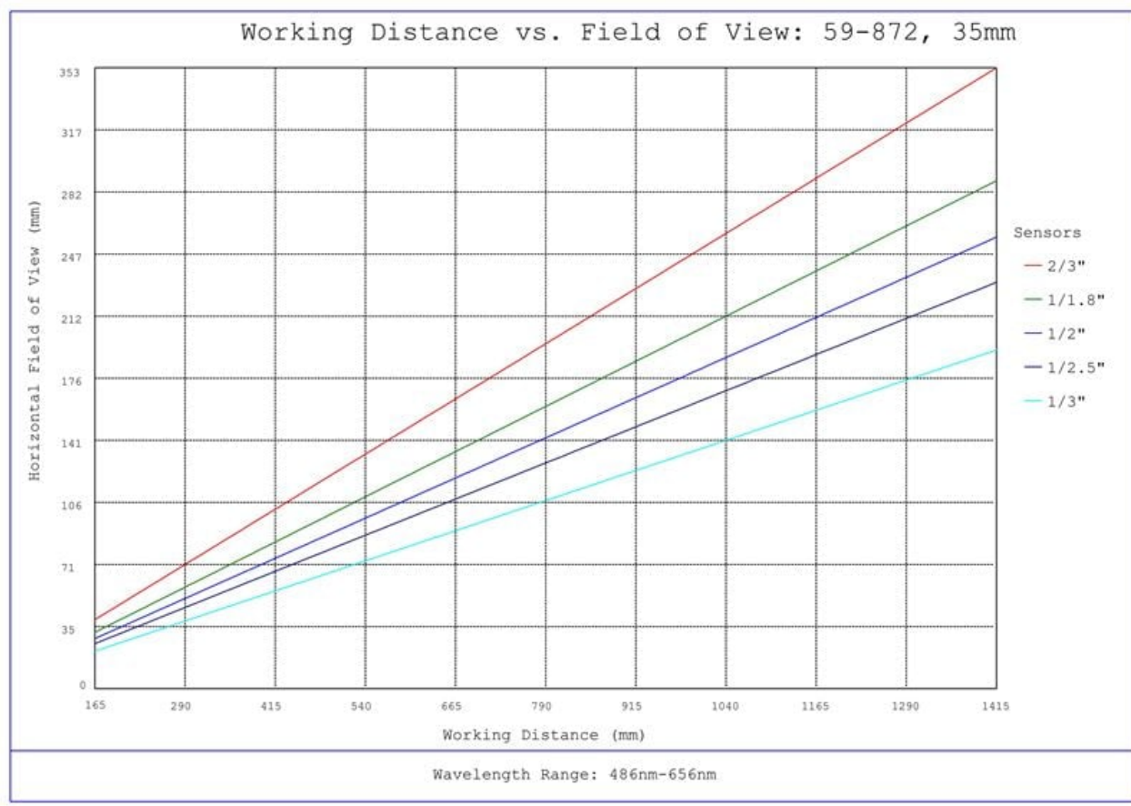
#59-872, 35mm C Series Fixed Focal Length Lens, Working Distance versus Field of View Plot
