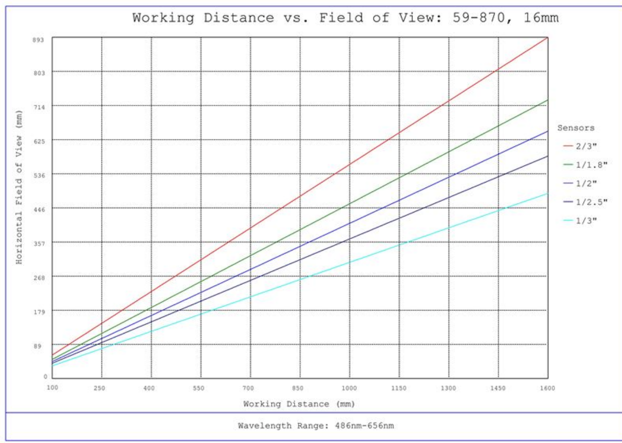
#59-870, 16mm C Series Fixed Focal Length Lens, Working Distance versus Field of View Plot
