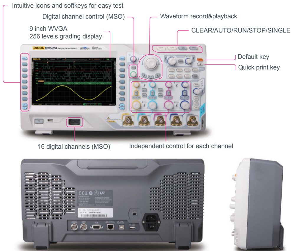
Product Dimensions: Width×Height×Depth = 440.0 mm×218.0 mm×130.0 mm Weight: 4.8 kg±0.2 kg (Without Package)
