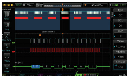
Deep memory depth for the digital channels, serial bus trigger and decoding on digital channels
