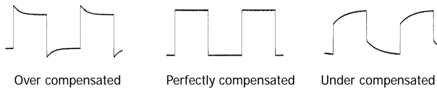
Figure 9 Probe Compensation
