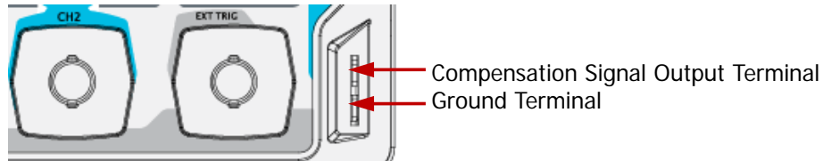
Figure 7 To Use the Compensation Signal
