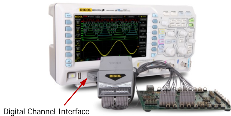
Figure 6 To Connect the Logic Probe
