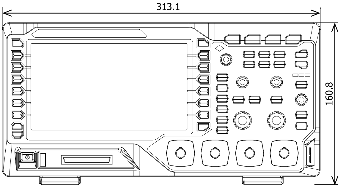
Figure 1 Front View
