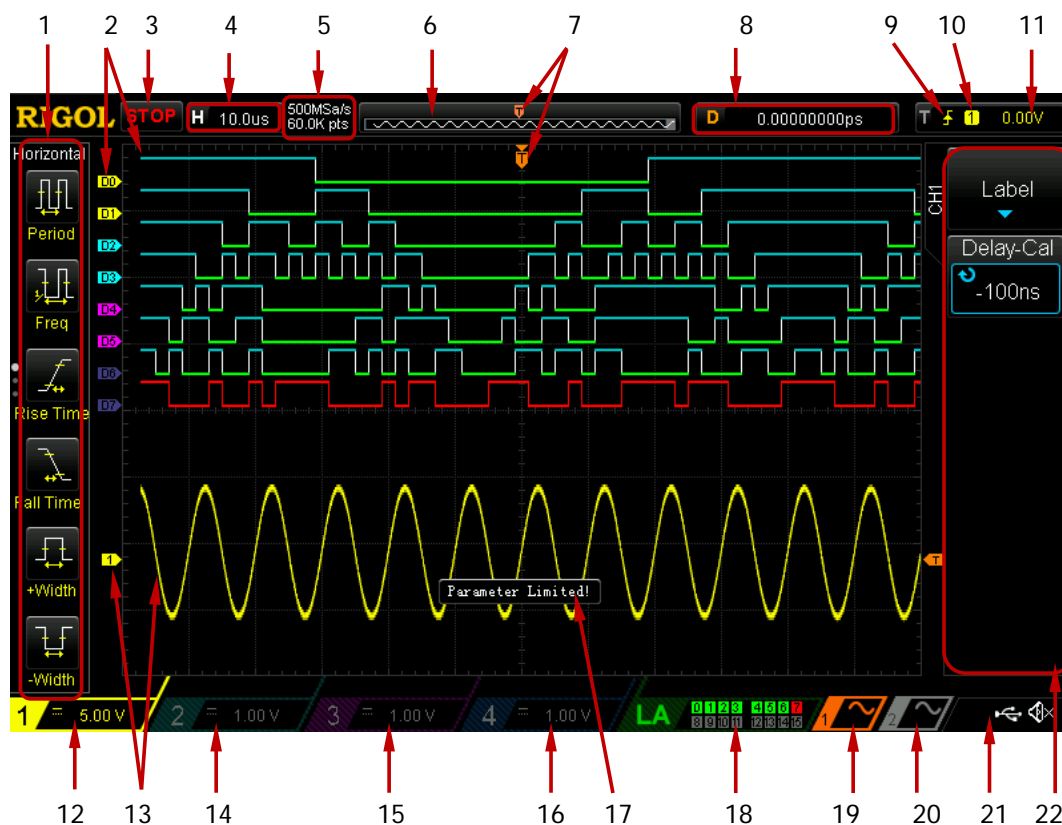
Figure 12 User Interface
