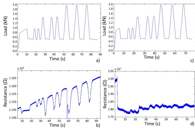
Fig. 7. Load applied during electromechanical tests with increasing loads and output of the brick sensors with carbon nano inclusions (a and b) and without fillers (c and d), under a stabilized voltage.
