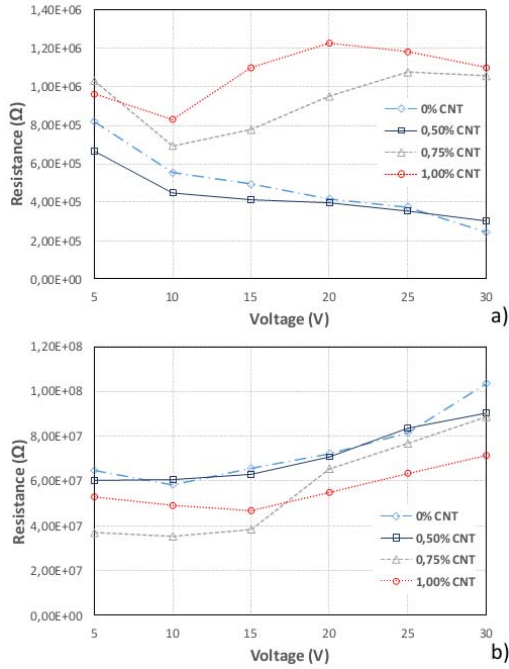
Fig. 6. Electrical resistance of composite clay brick sensors with various amounts of carbon nanotubes after drying (a) and after burning (b) versus different levels of applied voltage
