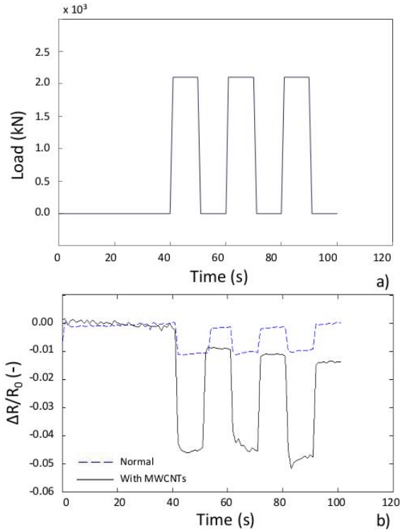
Fig. 8. Time history of the cyclical load applied during electromechanical tests (a) and normalized change in electrical resistance of the brick sensors with carbon nano inclusions and without fillers (b) under a square wave voltage (quantities are defined according to Eqs. (1) and (2)).
