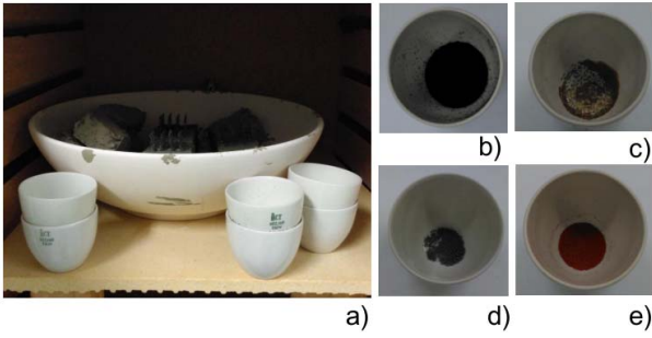
Fig. 5. Setup for the burning of samples and nanofillers (a); carbon nanotubes at room temperature (b); carbon black (c) carbon nanofibers (d) and carbon nanotubes (e) after burning at 900°C (c).
