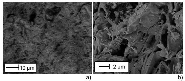
Fig. 2. SEM images of normal clay bricks after drying (a) and after burning at 900 °C (b)
