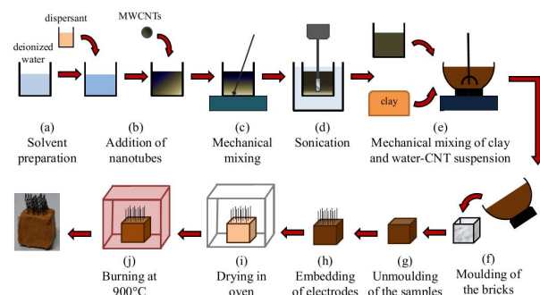
Fig. 1. Fabrication process of nanocomposite clay bricks.
