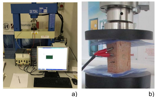
Fig. 4. Laboratory setup for electrical and electromechanical cyclical tests for sensing detecting (a) and a detailed view of the setup during an electromechanical test with increasing loads (b)
