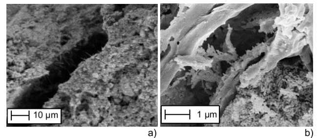
Fig. 3. SEM images of nanocomposite clay bricks after drying (a) and after burning at 900 °C (b)
