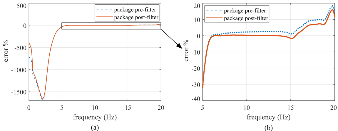
Figure 12. Pre and post filtering frequency domain error percentage in the bandwidth of: (a) 0-20 Hz; (b) 5-20 Hz.
