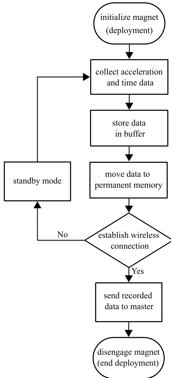
Figure 5. Sensor package deployment mission algorithm breakdown.
