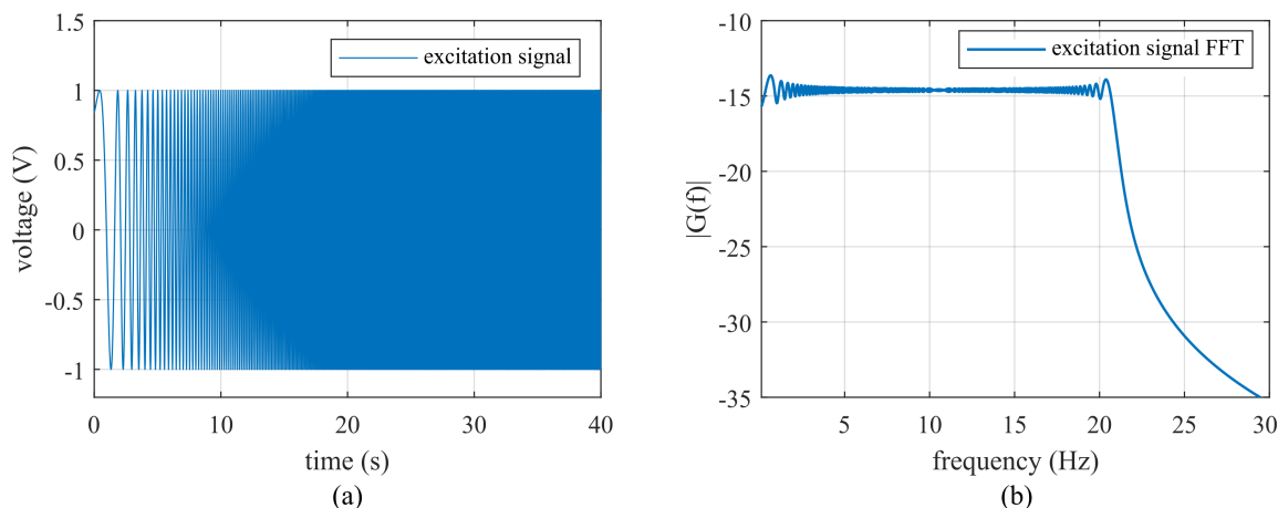
Figure 8. Normalized Chirp excitation signal: (a) time domain; (b) frequency domain plots.
