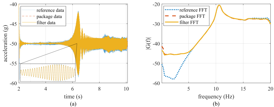
Figure 11. Structure test comparison between pre and post filter performance in the: (a) time domain; (b) frequency domain with respect to a reference accelerometer.
