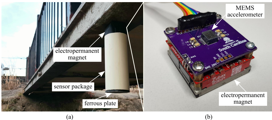
Figure 1. (a) Sensor package deployment under a pedestrian bridge, (B) MEMS accelerometer onboard the sensor package.
