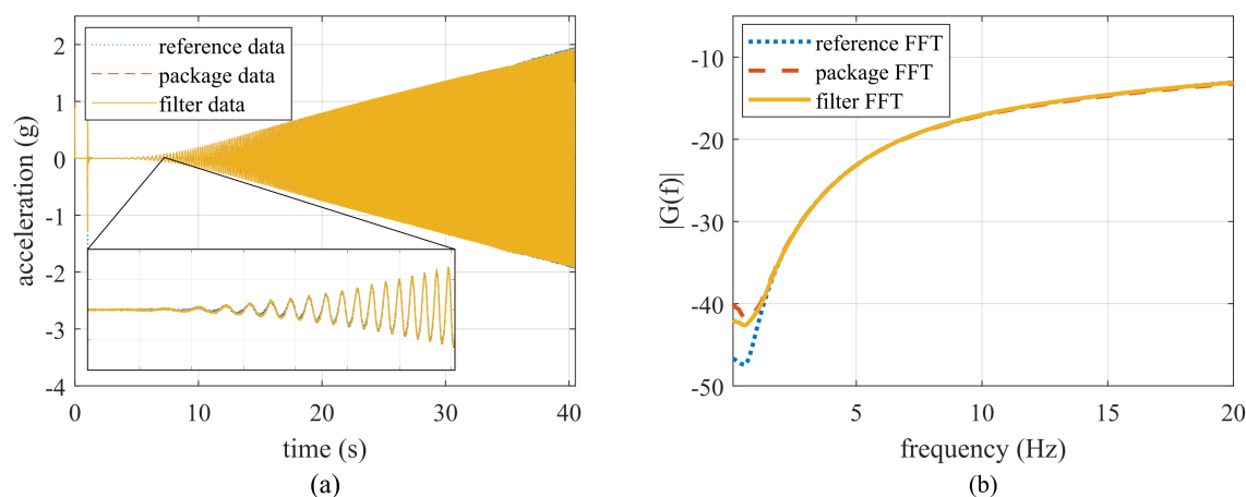
Figure 9. Benchmark experiment comparison between pre and post filter performance in the: (a) time domain; (b) frequency domain with respect to a reference accelerometer.
