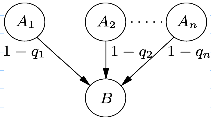
Fig. 3.25 (Independence of causal influence)
